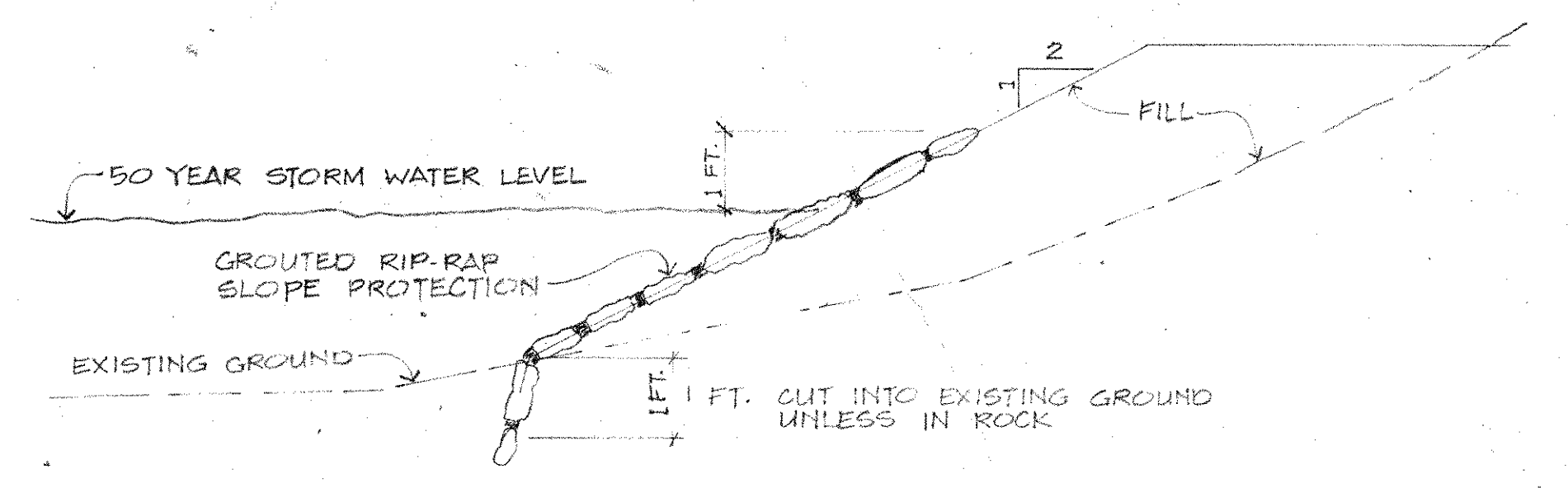
TYPICAL SLOPE PROTECTION ALONG GULCH NOT TO SCALE
