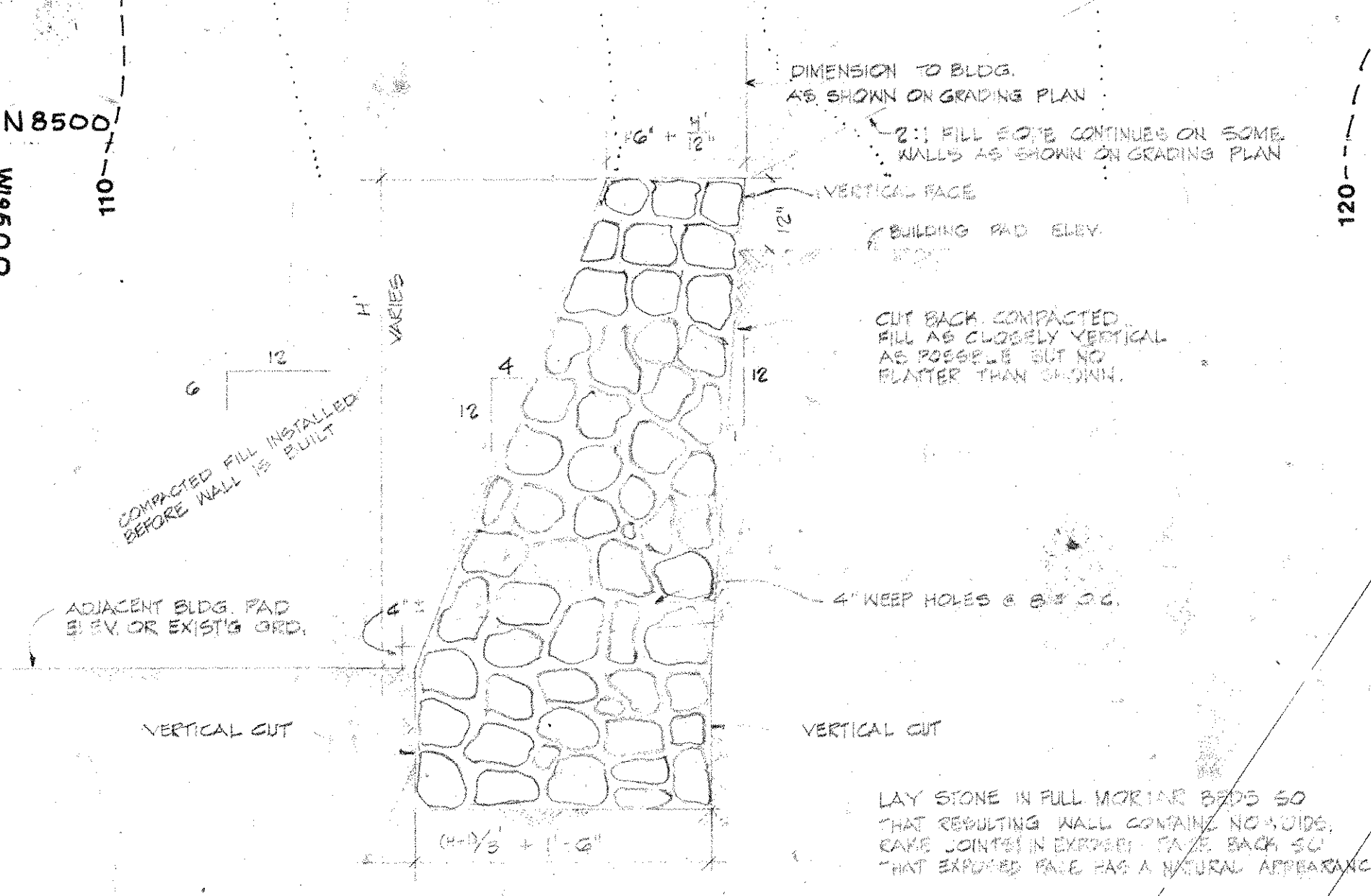
TYPICAL SECTION ROCK MASONRY WALL SCALE: 1/4" = 1'-0"
